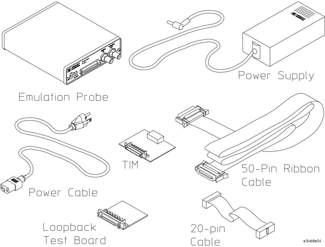
Equipment Supplied with Emulation Probe
